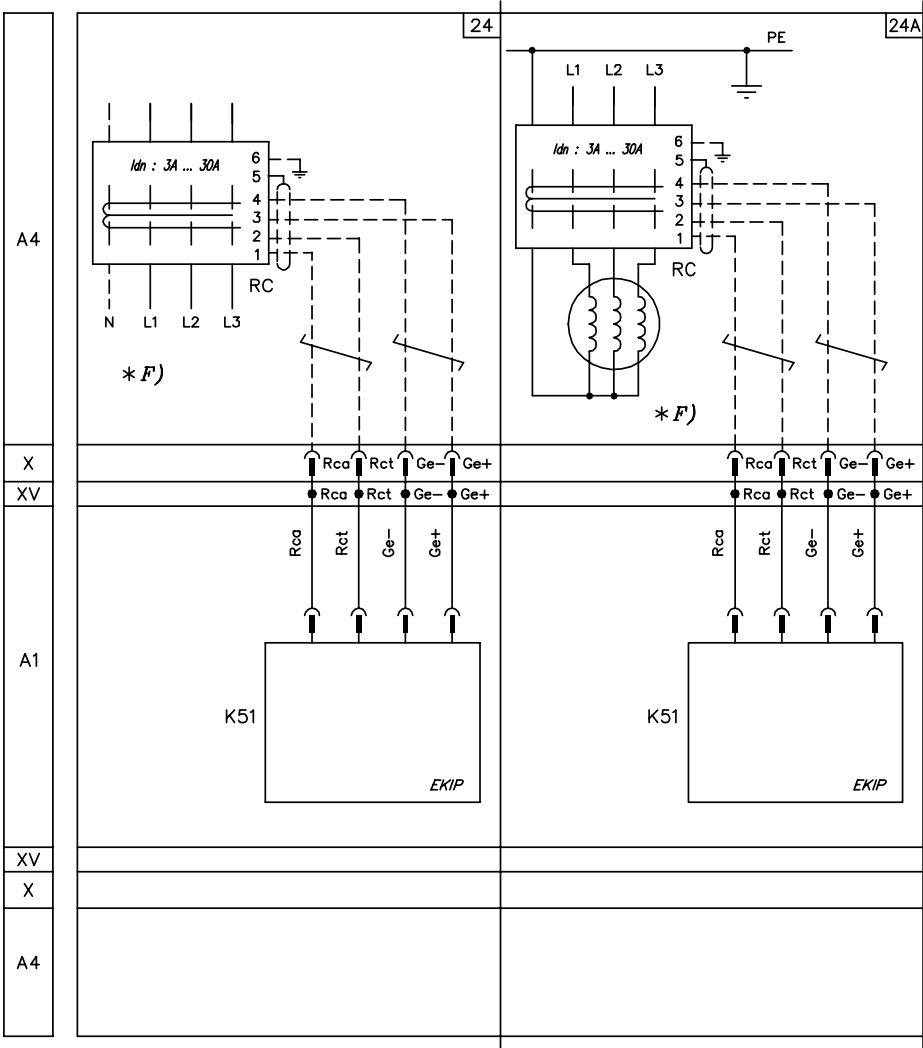
24) Rc residual current protection sensor input (ANSI 64 & 50NTD) 24a) Rc differential ground fault protection (ANSI 87N)
